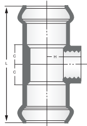
Tap Service Tee (NPT Outlet)
